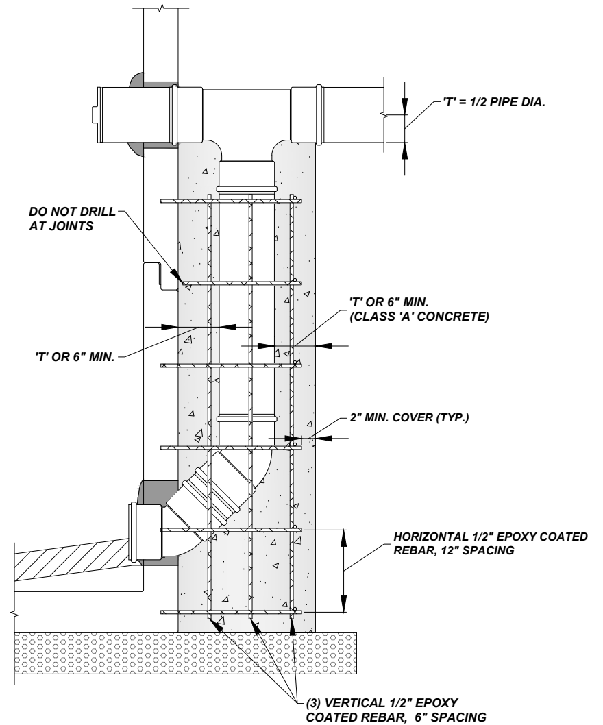
SECTION VIEW
