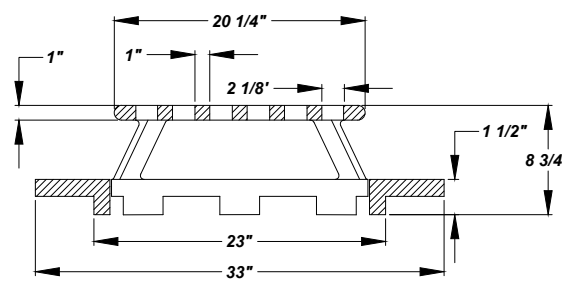
DITCH/DRYWELL CASTING DETAIL NEENAH R-4341-A
