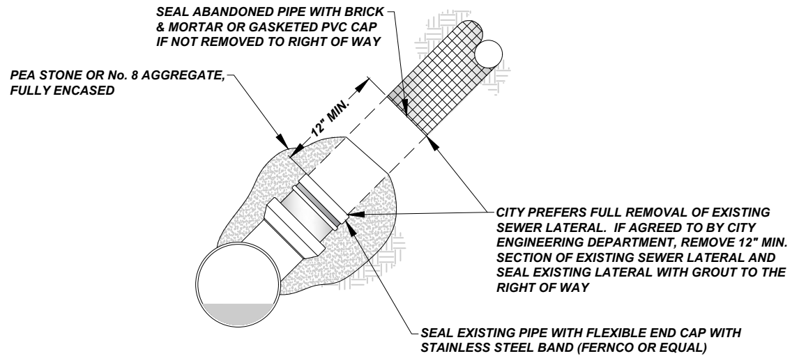
PROFILE VIEW
