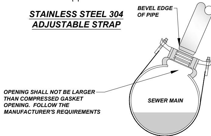
SEWER SADDLE CONFORMING TO PIPE
