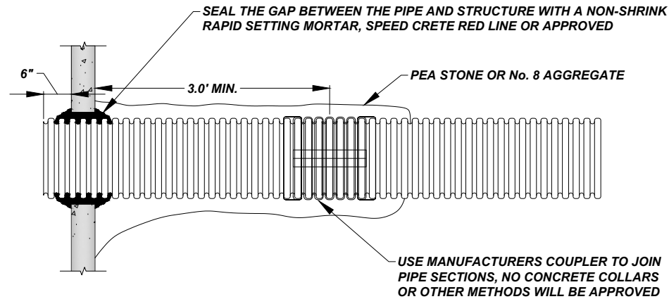
CORRUGATED COUPLER CONNECTION
