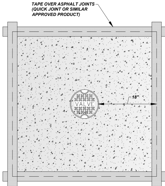
SAW CUT - PLAN VIEW
