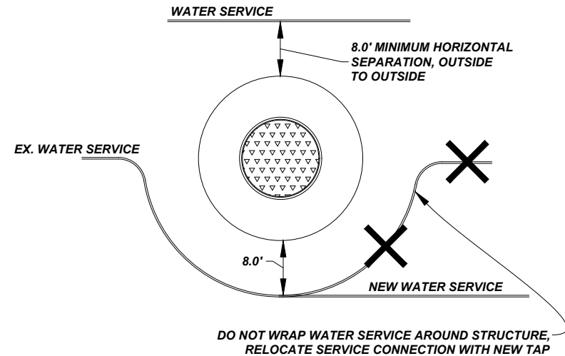
WATER SERVICE AND STRUCTURE CONFLICT
